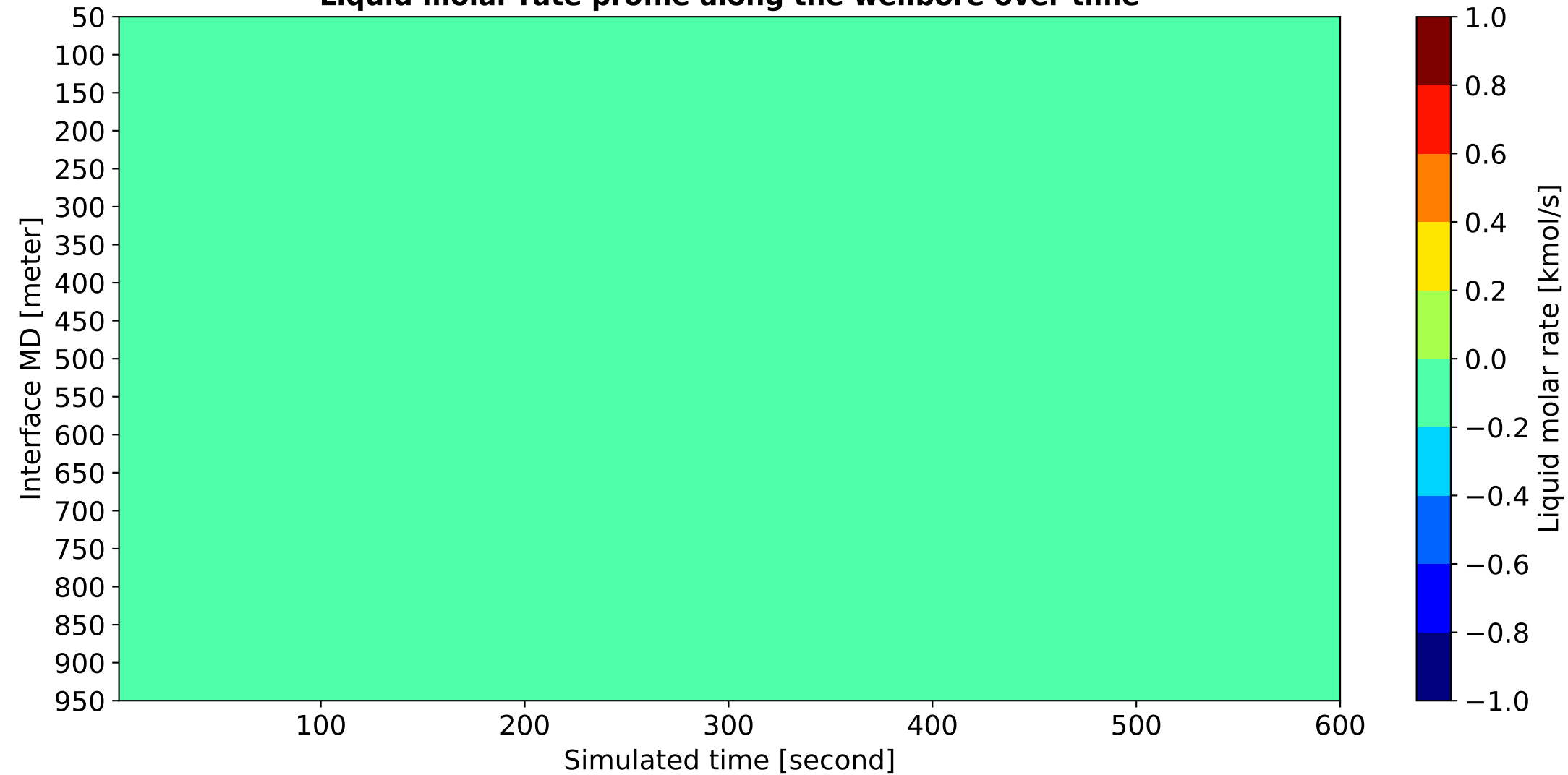
Liquid molar rate profile along the wellbore over time
